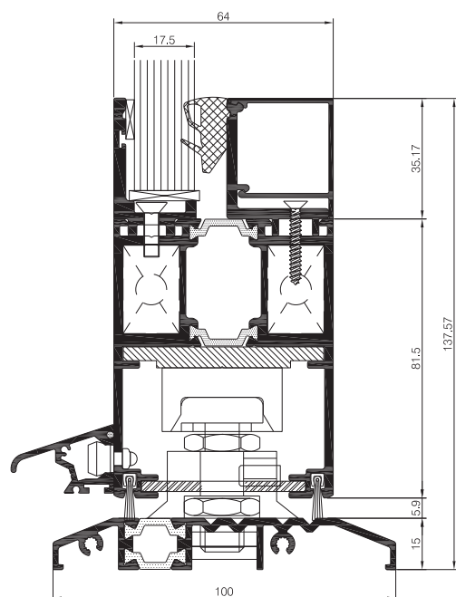
General Arrangement showing Comar 7P.i CD with a low-rise thermally broken sill option
